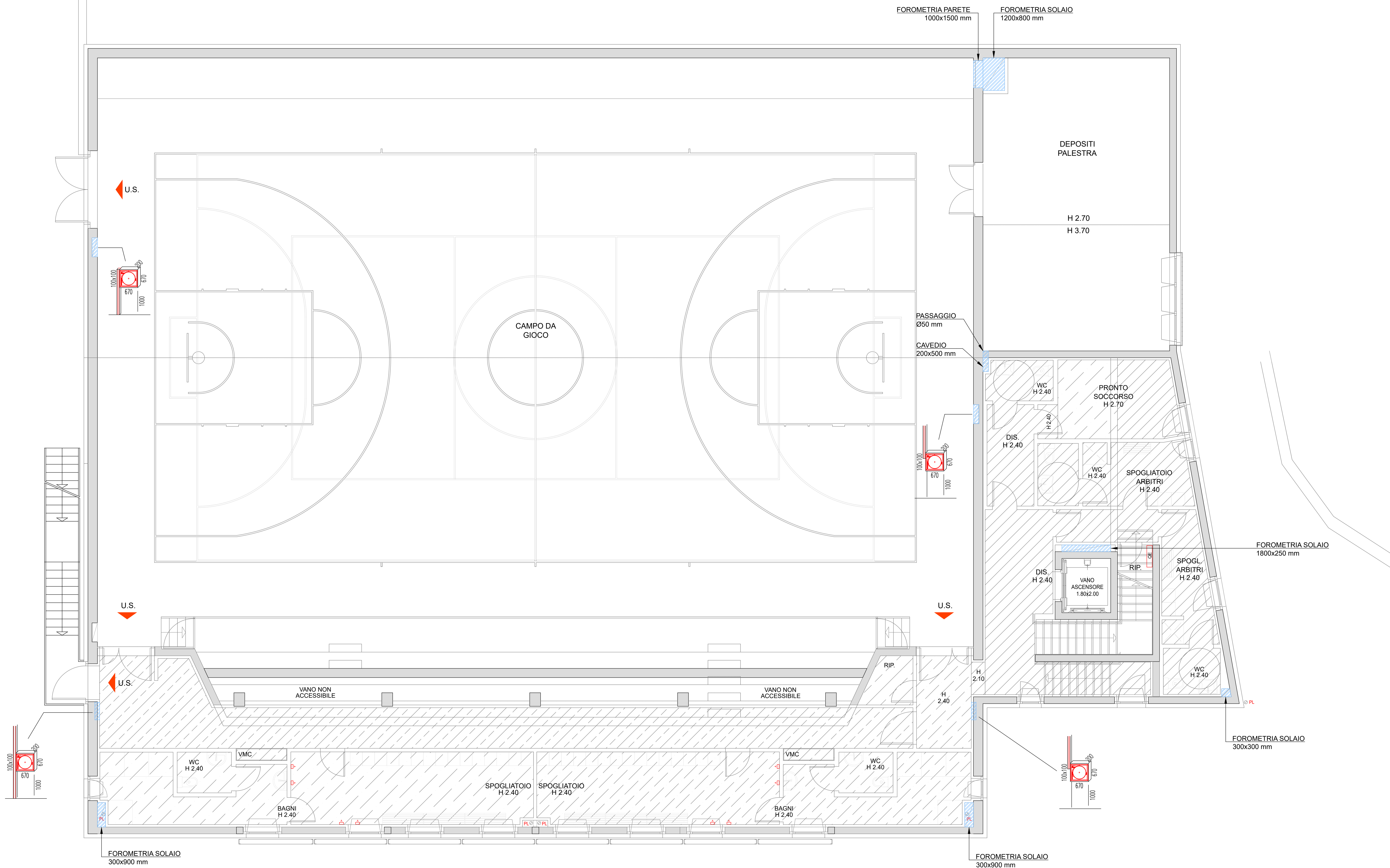
PIANTA PIANO +6,10
